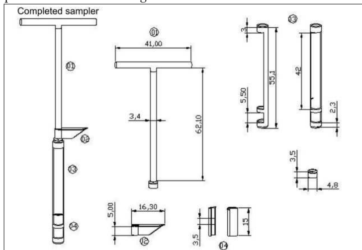
Figure 2. Scheme with dimensions of the sampler Jadoski model, version 01, developed for the sampling of structured soil samples with a volumetric ring.
