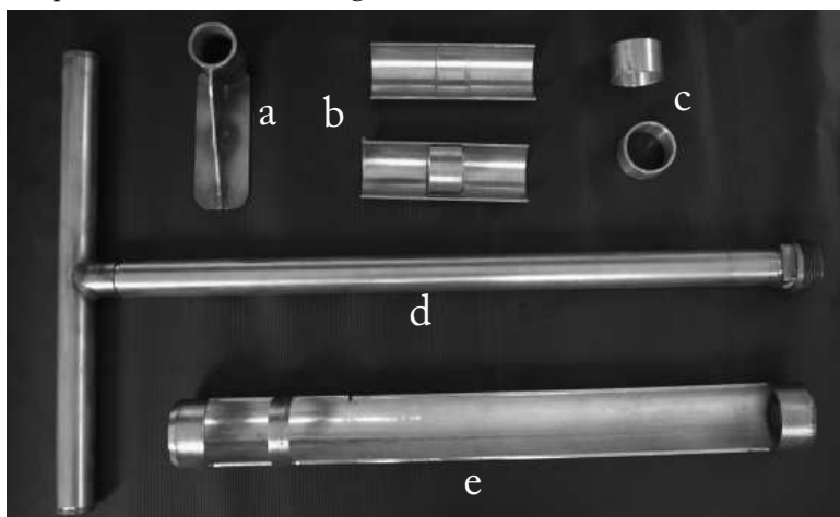
Figure 3. Photograph of the components of the sampler Jadoski model, version 1.0 developed for the sampling of structured soil samples with a volumetric ring.
